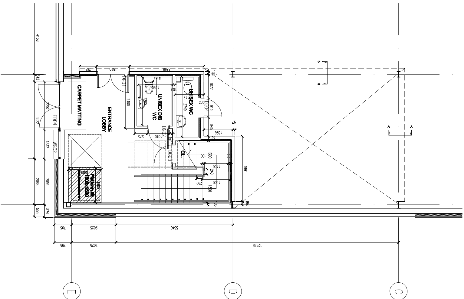
UNIT E GROUND FLOOR OFFICE CORE LAYOUT
